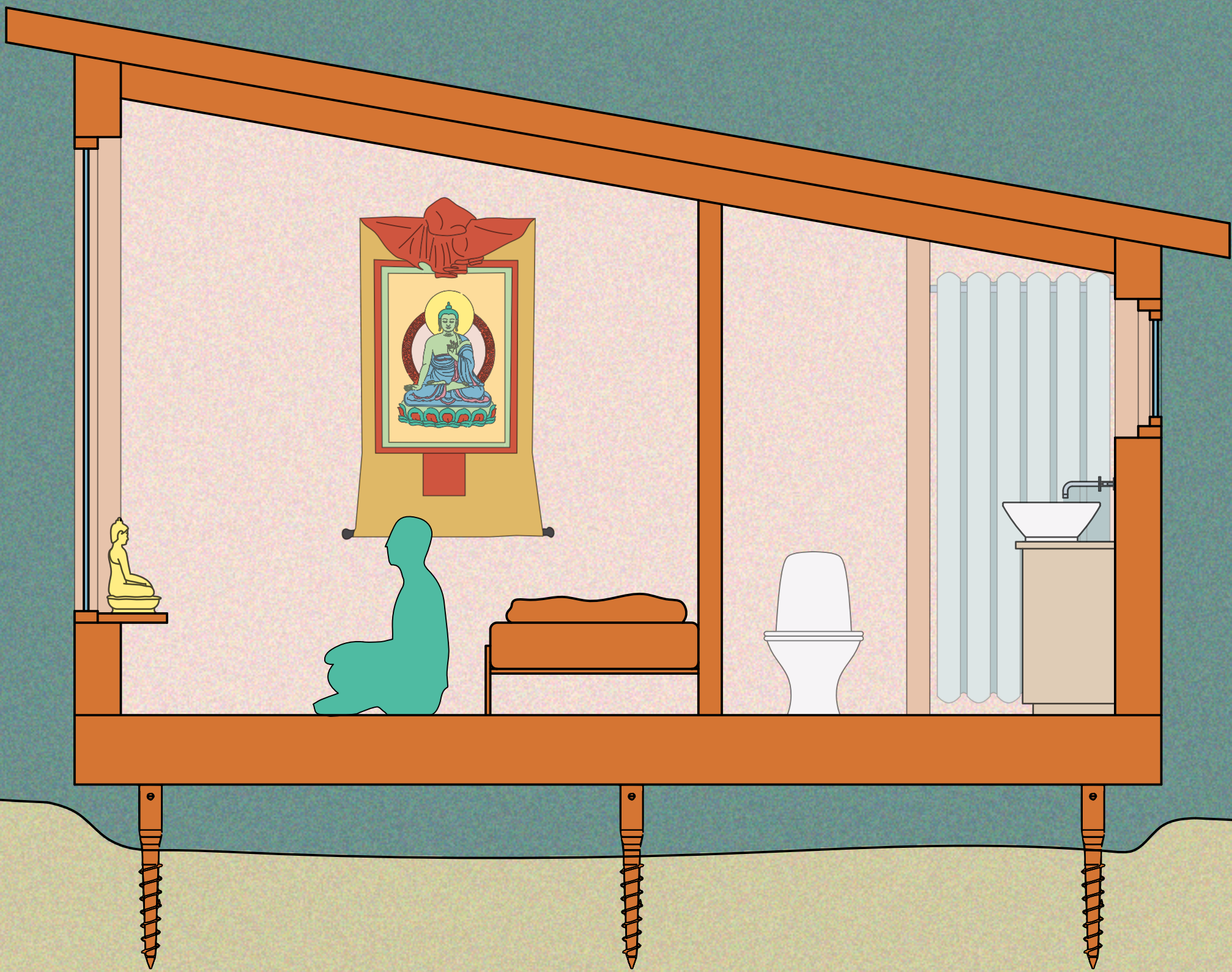
Section 1:50
